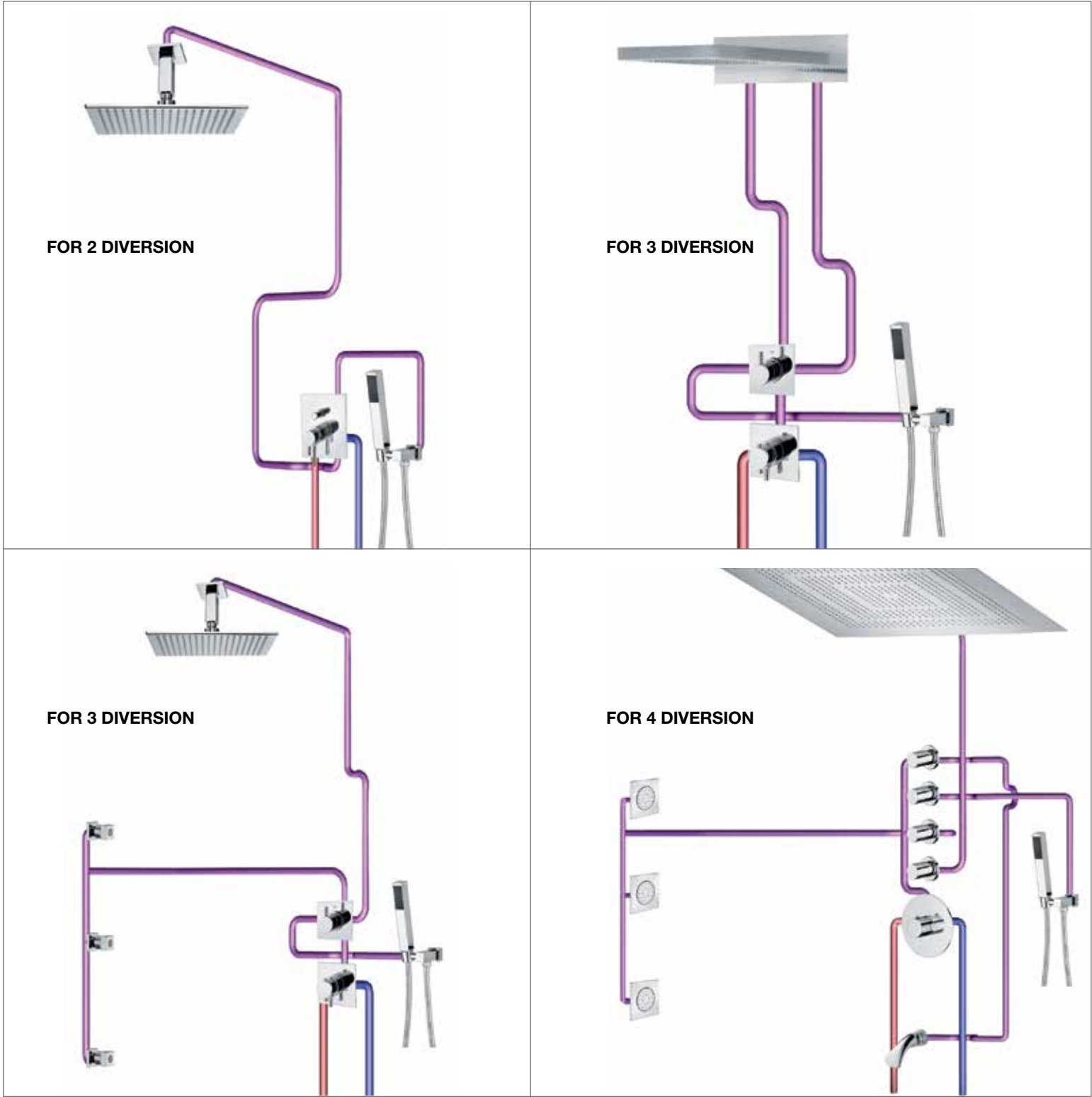
RECOMMENDED PIPING LAYOUT
